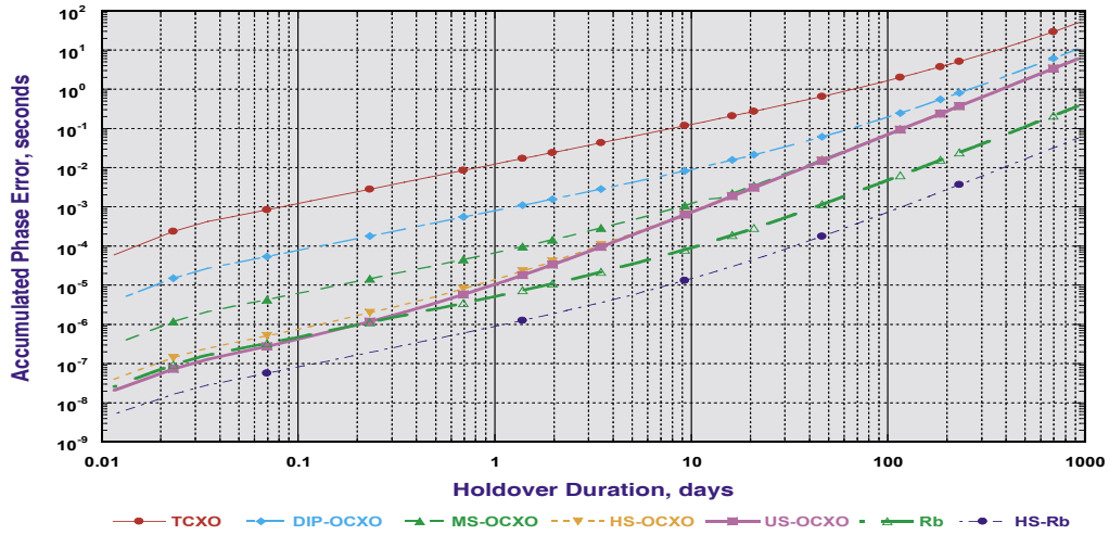
Holdover Performance - Oscillator Options Typical, 5° C Max Delta, 7.5° C/Hr Max SlewRate
